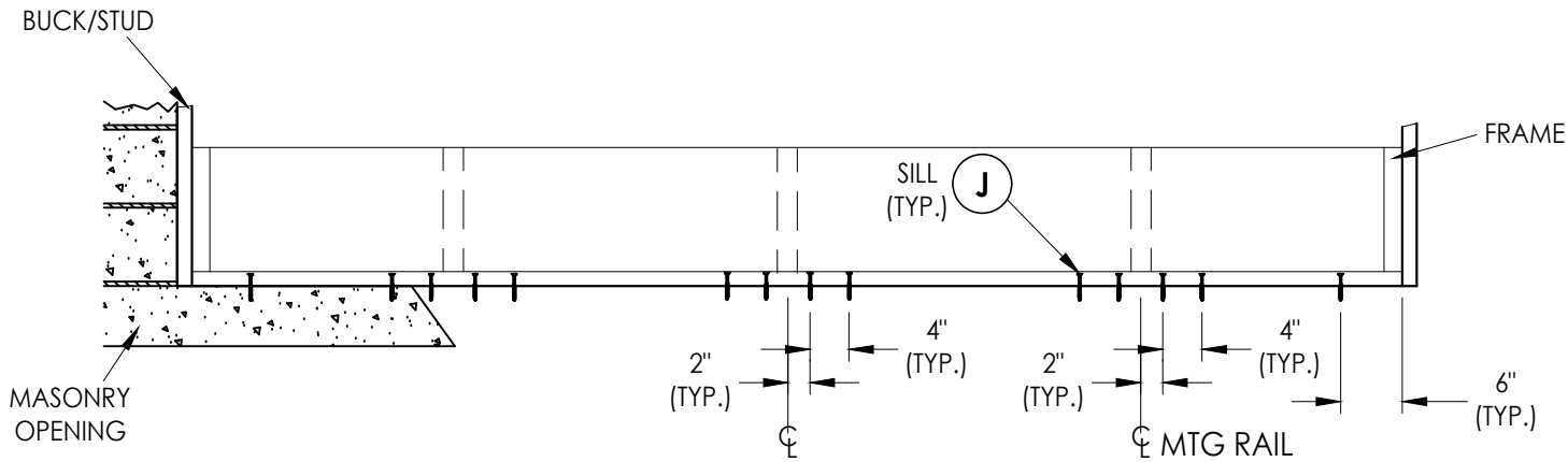
ALTERNATE FRAME ANCHORING DIRECT TO MASONRY @ SILL
